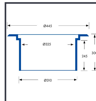
ECO-315-GR D400 Rund karm & rist VVS nr.: 22.1117.231
