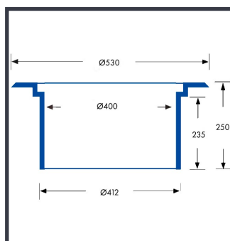
ECO-425-GR D400 Rund karm & rist VVS nr.: 22.1117.242
