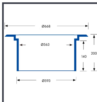
ECO-600-GR D400 Rund karm & rist VVS nr.: 22.1117.260
