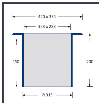
ECO315-RTLs Rendestensrist VVS nr.: 22.1129.831
